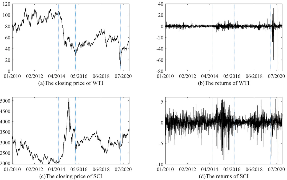
Fig. 2. The closing price and return series of WTI and SCI.
