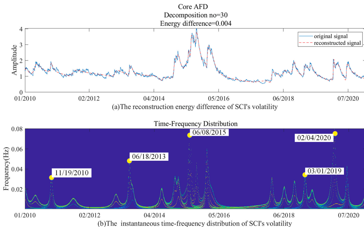
Fig. 3. The energy difference and the instantaneous time-frequency distribution of SCI's volatility.
