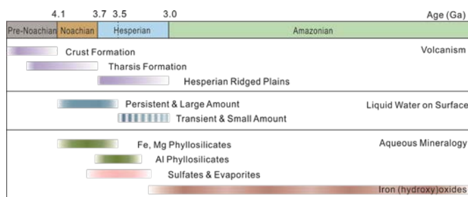
Timeline of some major events on the Martian surface (Du et al, Earth-Science Reviews , 2023).
